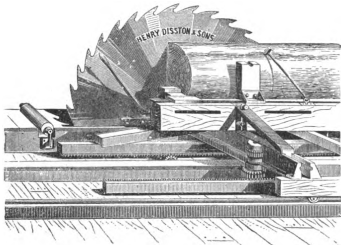
Left Hand Saw.
